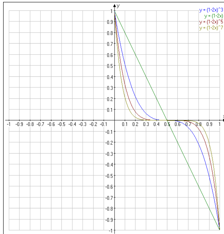
Figure 2 Graph showing the levels of e-trust provided by using the equation y = (1 - 2x)^n with different powers.
